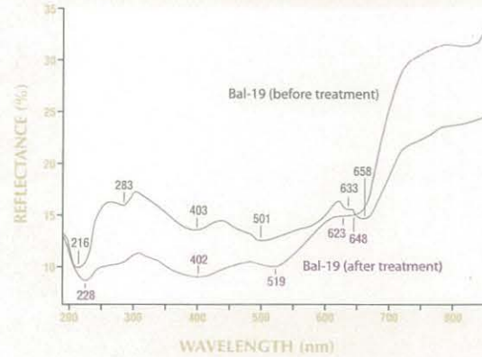
Figure 11. After treatment, the baseline of the UV-Vis-NIR reflectance spectrum of sample Bal-19 increased in general absorption toward the low-wavelength (high-energy) side; this appears to be a useful feature for identifying this type of "chocolate pearl." Also, absorption bands associated with organic components became less distinct.
