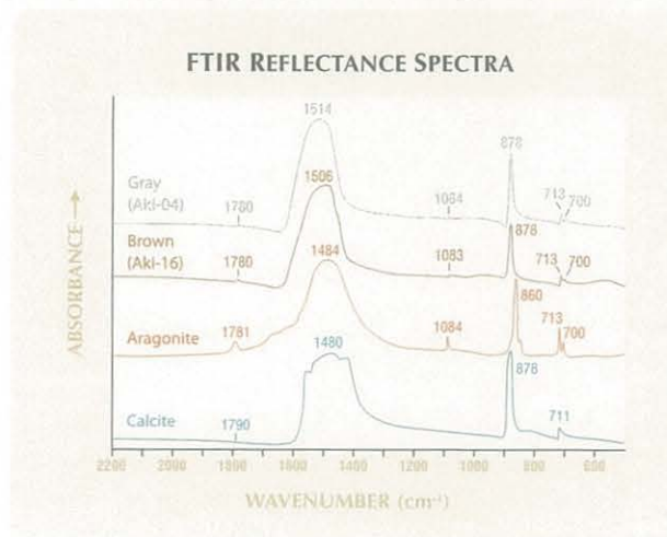
Figure 6. The mid-infrared reflectance spectra of the NCTCPs are similar to the spectrum of aragonite, in particular with the occurrence of a peak at 1084 \text{cm}^{-1} . However, the peak at 878 \text{cm}^{-1} for the NCTCPs is much higher in position than the 860 \text{cm}^{-1} peak in aragonite, and occurs at nearly the same position as seen in calcite. Gray and brown NCTCPs examined for this study displayed identical absorption features.
