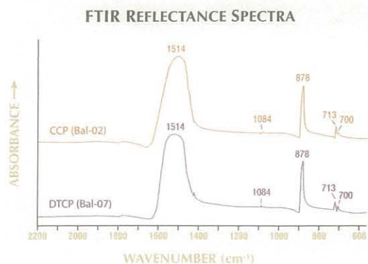
Figure 7. The mid-infrared absorption spectra of the CCPs and DTCPs were nearly identical to those of the NCTCPs in figure 6.
