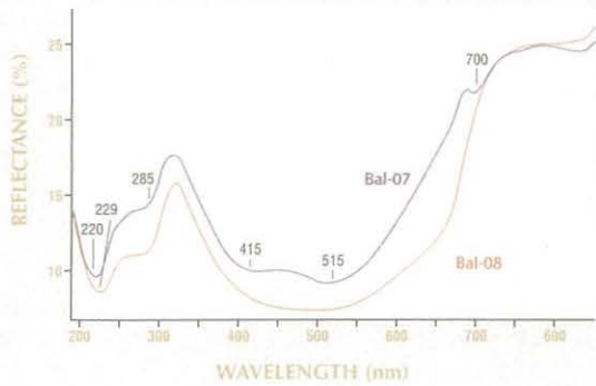
Figure 10. The UV-Vis-NIR reflectance spectra of these two DTCPs are very different from those of the NCTCPs and the CCPs. The spectra are dominated by a broad absorption band that ranges from ~320 to ~700 nm and is centered at ~500 nm.
