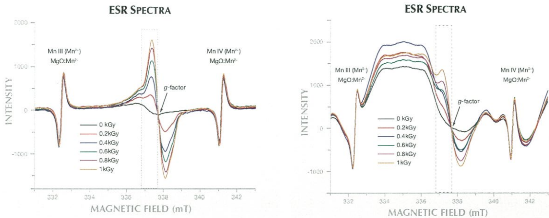
Figure 5. These ESR spectra show a South Sea cultured pearl's nacre (left) and nucleus (right) before and after irradiation up to 1 kGy. These spectra were obtained for a single cultured pearl irradiated with different doses. \text{CO}_2^- radicals appeared as irradiation doses increased in both the nacre (left) and nucleus (right). Nucleus spectra (right) show a large unassigned signal in the 333–337 mT range, both before and after irradiation.
