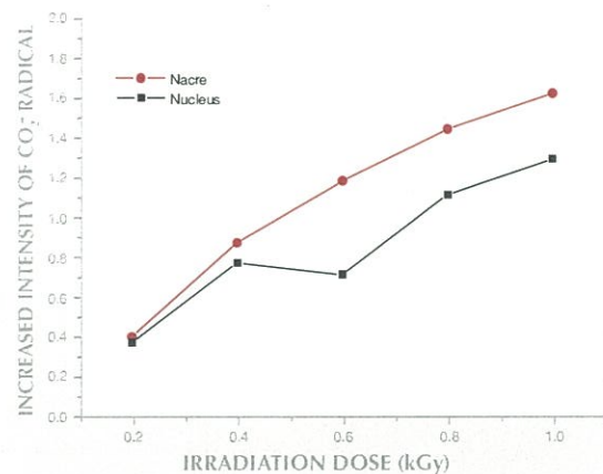
Figure 7. Normalizing the CO 2 - radical intensity of figure 5 shows that the radicals' intensity increases depending on irradiation dose, even though the CO 2 - radical of the nucleus (bead) decreased at 0.6 kGy.
