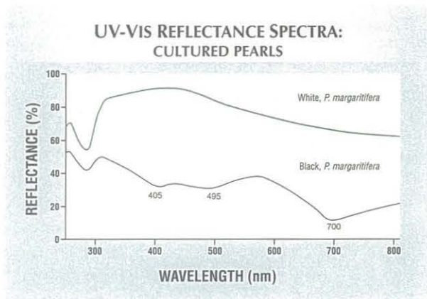
Figure 5. Reflectance spectra are shown here for white and black cultured pearls from the P. margaritifera . The absorption features measured for the black sample at 405, 495, and 700 nm are characteristic of black cultured pearls from this species.
