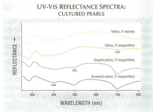
Figure 6. Reflectance spectra for yellow, grayish yellow, and brownish yellow cultured pearls from P. margaritifera are compared here with the spectrum for a yellow cultured pearl from P. maxima . Note the similarity in absorption features in the UV region between 330 and 460 nm for the “pure” yellow samples, as compared to the grayish and brownish yellow samples. All three P. margaritifera samples exhibit the absorption feature at 700 nm, which is absent from the yellow P. maxima sample and also the white P. margaritifera sample shown in figure 5.
