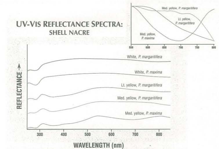
Figure 4. These reflectance spectra are for white and yellow nacre samples taken from the shells of P. margaritifera and P. maxima . The spectra for respective colors are similar in the 330 to 550 nm region, but often differ from 550 to 800 nm. The inset vertically expands this region to illustrate how the weak absorption feature at 700 nm exhibited by the darker P. margaritifera sample is distinctly different from the broad absorption often seen in the P. maxima samples.
