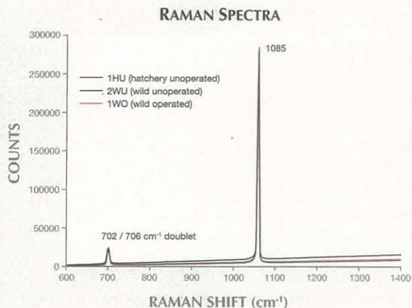
Figure 34. Three representative Raman spectra were gained from pearls produced by a P. maxima hatchery-reared shell, a wild unoperated P. maxima shell, and a wild operated P. maxima shell. Each showed virtually identical spectral features that were consistent with aragonite. The representative samples are the same as those used for the PL spectra (figure 35).
