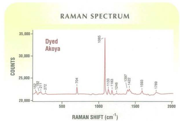
Figure A-2. In this Raman spectrum of an orangy yellow Akoya cultured pearl, the series of peaks above 1085 \text{cm}^{-1} indicate treatment with an organic dye.
