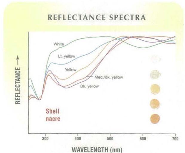
Figure 6. These reflectance spectra of five shell nacre samples—ranging from white through dark yellow—show increasing absorption from 330 to 460 nm as the color intensifies. Note in particular the increasing absorption in the UV region from 330 to 385 nm.
