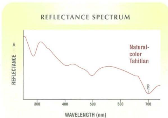
Figure A-3. In a UV-Vis (ultraviolet-visible) reflectance spectrum, an absorption maximum at 700 nm is characteristic of natural-color black cultured pearls from the Pinctada margaritifera oyster.
