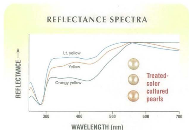
Figure 9. The reflectance spectra of the heat-treated yellow cultured pearls revealed very weak or no absorption in the 330–385 nm region. The presence of a weak UV absorption feature around 345 nm suggests that the orangy yellow cultured pearl exhibited some natural yellow coloration prior to treatment.
