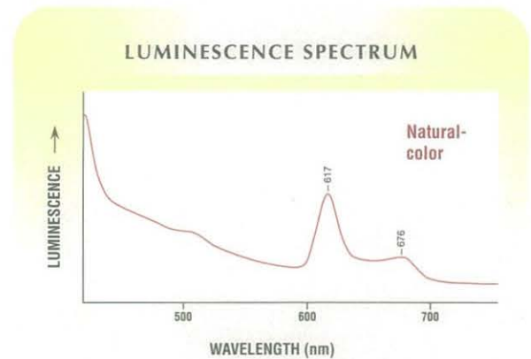
Figure A-4. This luminescence spectrum of a cultured black pearl from Pinctada margaritifera shows fluorescence peaks at 617 and 676 nm due to porphyrins, which are responsible for the reddish brown fluorescence to 365 nm UV or 405 nm blue light.
