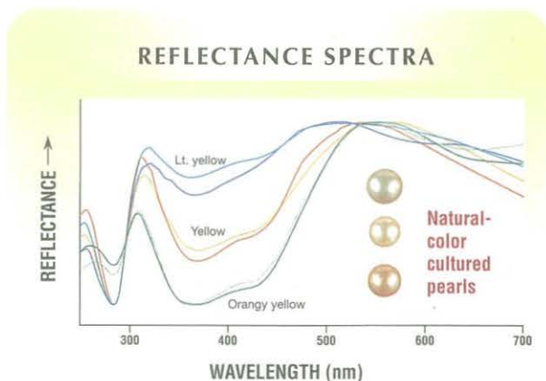
Figure 8. As was the case with the shell nacre samples, the reflectance spectra of the natural-color yellow cultured pearls showed increasing absorption in the 330–460 nm region with greater saturation of color.
